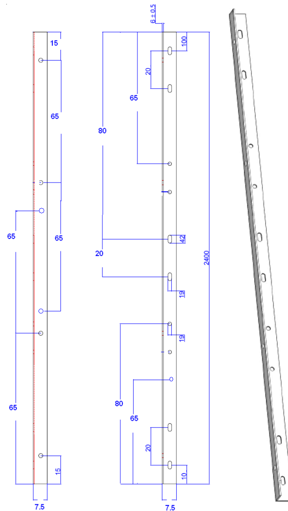
DIAGONAL HIERRO PLATINA 32X6 mm. X 0.7 mts.
